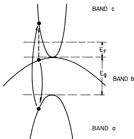
FIG. 2. Band structure of gray tin near the \Gamma point of the Brillouin zone. The two transitions that give rise to interband electronic Raman scattering considered in this paper are indicated. Dashed arrow indicates the net electronic excitation.
